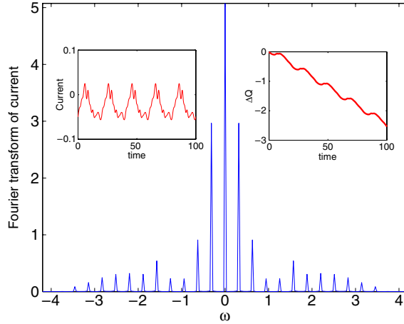
Figure 3. Fourier transform of the current (in units of q ) versus frequency for oscillating potentials at eight sites, with a = 2 , \omega = \pi/10 and k_F = \pi/4 for a system with 638 sites ( N_L = 315 ). The left and right insets show the current and charge transferred versus time.
