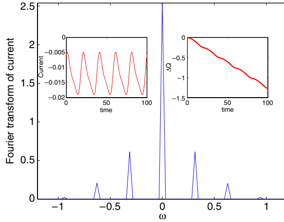
Figure 2. Fourier transform of the current (in units of q ) versus frequency for oscillating potentials at eight sites, with a = 0.2 , \omega = \pi/10 and k_F = \pi/4 for a system with 638 sites ( N_L = 315 ). The left and right insets show the current and charge transferred versus time.
