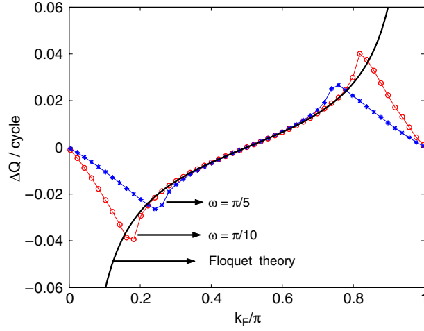
Figure 1. Charge transferred (in units of q ) per cycle from left to right versus the Fermi wavenumber for an oscillating potential at two sites, with a_1 = a_2 = 0.2 , \phi_2 - \phi_1 = \pi/2 , and \omega = \pi/10 (circles) and \pi/5 (stars) for a system with 202 sites ( N_L = 100 ). The solid line shows the results obtained using second-order Floquet scattering theory in the limit \omega \rightarrow 0 .
