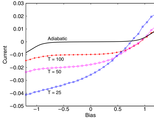
Figure 9. Current (in units of q ) versus bias for different frequencies (with T = 2\pi/\omega ) for oscillating potentials at eight sites, with a = 2 and k_F = \pi/4 for a system with 428 sites ( N_L = 210 ).
