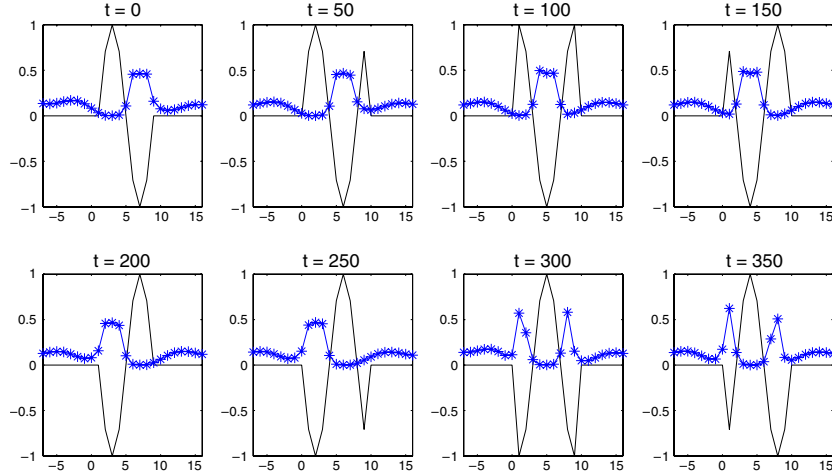
Figure 5. Electron numbers (stars) and potentials at 24 sites in and on two sides of the scattering region (sites 1–8) at eight equally spaced times in one cycle, for potentials oscillating with a = 2 , \omega = \pi/200 and k_F = \pi/8 for a system with 1618 sites ( N_L = 805 ). The scale on the y-axis indicates both the electron number and the potential (divided by 2) at each site.
