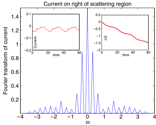
Figure 7. Fourier transform of the current (in units of q ) on the right of the scattering region versus frequency for oscillating potentials at eight sites, with a = 2 , \omega = \pi/10 and k_F = \pi/4 for a system with 428 sites ( N_L = 210 ). The left and right insets show the current and charge transferred versus time.
