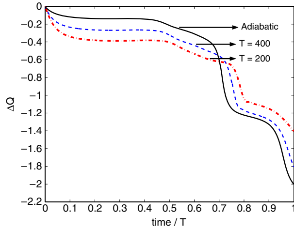
Figure 4. Charge transferred (in units of q ) from left to right versus time during one cycle (with period T = 2\pi/\omega ) for oscillating potentials at eight sites, with a = 2 , k_F = \pi/8 , and \omega = \pi/100 (dash-dot), \pi/200 (dashed), and tending to zero (solid line).
