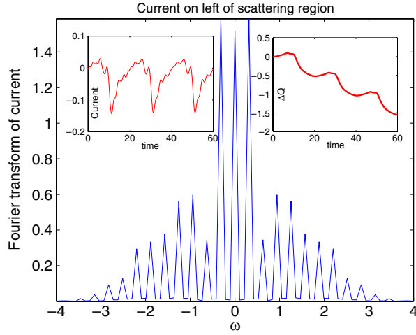
Figure 6. Fourier transform of the current (in units of q ) on the left of the scattering region versus frequency for oscillating potentials at eight sites, with a = 2 , \omega = \pi/10 and k_F = \pi/4 for a system with 428 sites ( N_L = 210 ). The left and right insets show the current and charge transferred versus time.
