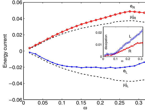
Figure 8. Energy currents e_L and e_R on the left and right of the scattering region versus frequency for oscillating potentials at eight sites, with a = 2 and k_F = \pi/4 . The curves marked as \mu j_L and \mu j_R show the product of the chemical potential with the charge currents j_L and j_R on the left and right. The inset shows the heat current on the left and right versus frequency; these are given by e_L - \mu j_L and e_R - \mu j_R respectively.
